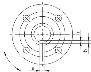
DN600/1000
