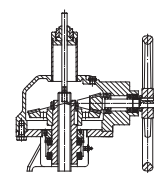
Limit switches
